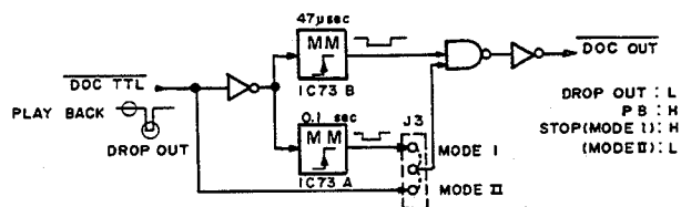
Fig. 1-17 DOC circuit
