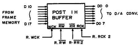
Fig. 1-11 Post-1H buffer
